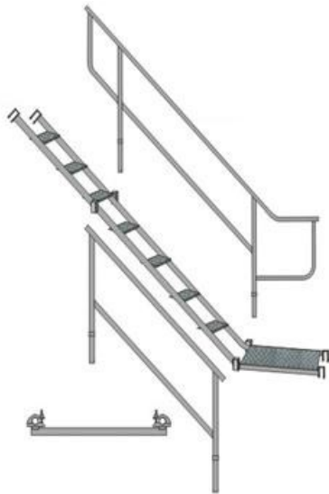
7' Internal Stairway Unit w/ Hand Rails (Starter bar sold separately)
