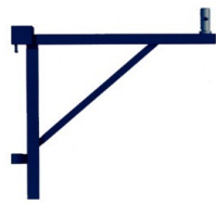
Side Bracket w/ Coupling Pin (angle iron) "Bell Hanger"
