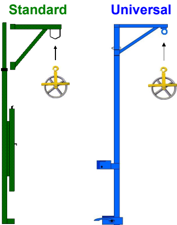
Hoist Arm & Bracket Specify style of Style (wheel not included)
